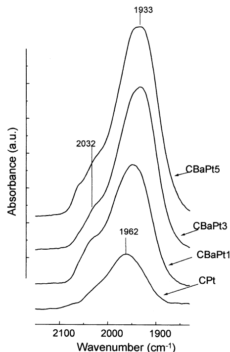
Figure 6. FTIR spectra of CO remaining on the CBaPt catalysts upon adsorption at room temperature and 4 kPa and subsequent evacuation at 523 K and 10^{-2} Pa.
